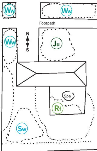
This plan shows different sections needed for a house garden irrigation system
